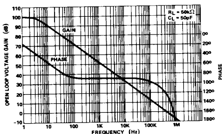
OPEN LOOP FREQUENCY RESPONSE
