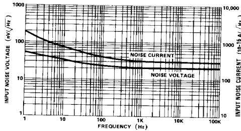
INPUT NOISE vs. FREQUENCY
