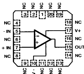
HA4-5141/883 (CERAMIC LCC) TOP VIEW
