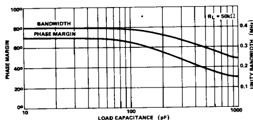
BANDWIDTH AND PHASE MARGIN vs. LOAD CAPACITANCE
