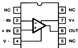
HA7-5141/883 (CERAMIC MINI-DIP) TOP VIEW
