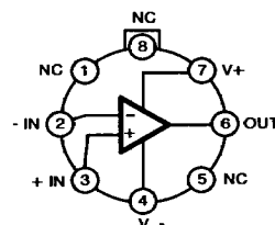
HA2-5141/883 (METAL CAN) TOP VIEW
