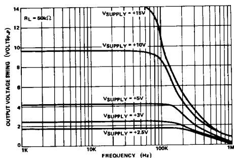
OUTPUT VOLTAGE SWING vs. FREQUENCY AND SINGLE SUPPLY VOLTAGE
