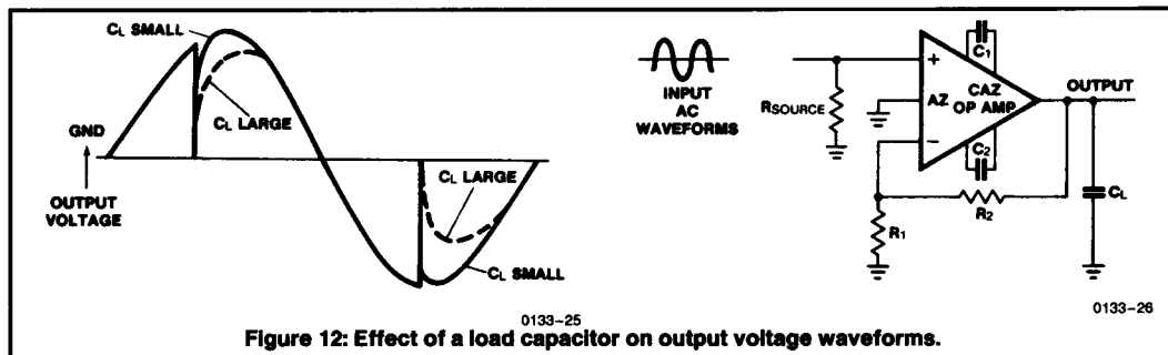
Figure 12: Effect of a load capacitor on output voltage waveforms.
