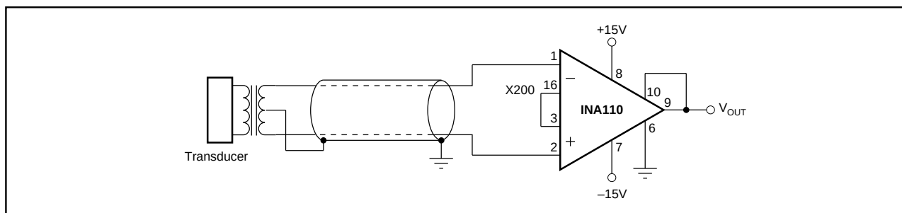
FIGURE 6. Transformer-Coupled Amplifier.
