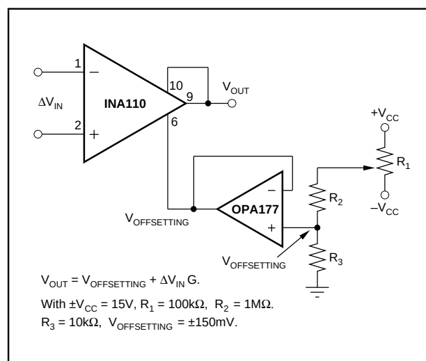
FIGURE 3. Output Offsetting.
