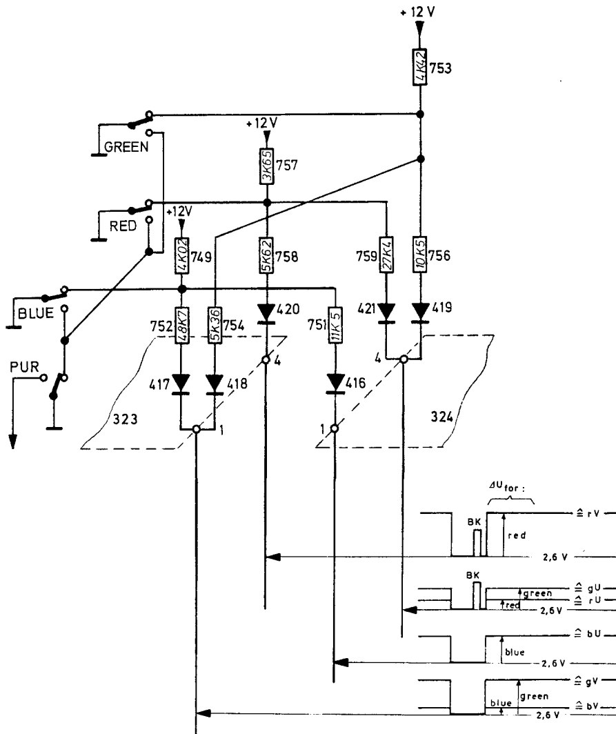
Fig. 19 Matrix of the monochrome pattern red, green and blue
