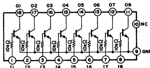
IC103, 106: AN6551, NJM4558S, BA715
