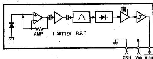
U101: GP1U501 (Remote Control Receptor)
