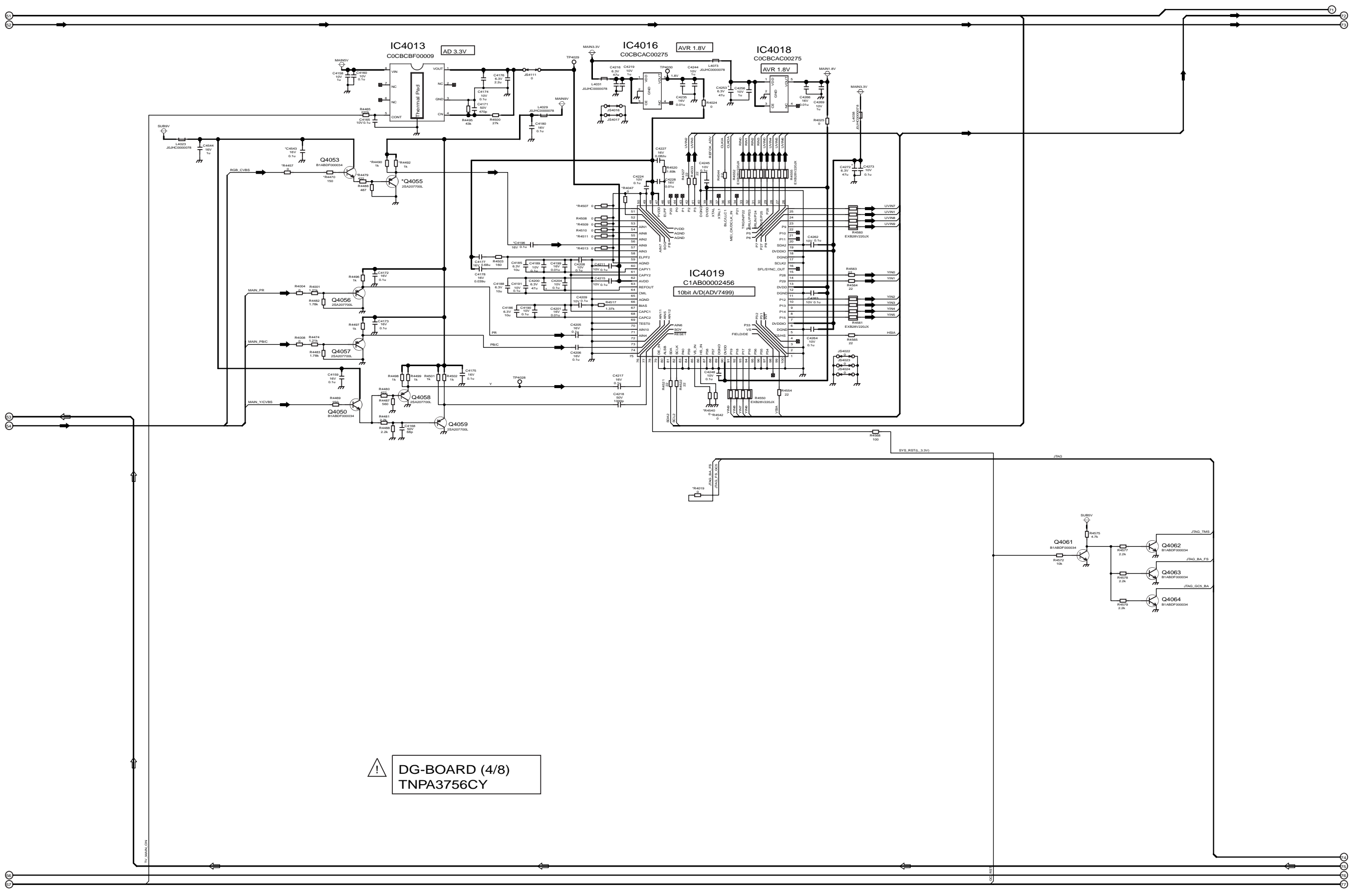
TH-42PA60L DG-Board (4 of 8) Schematic Diagram
