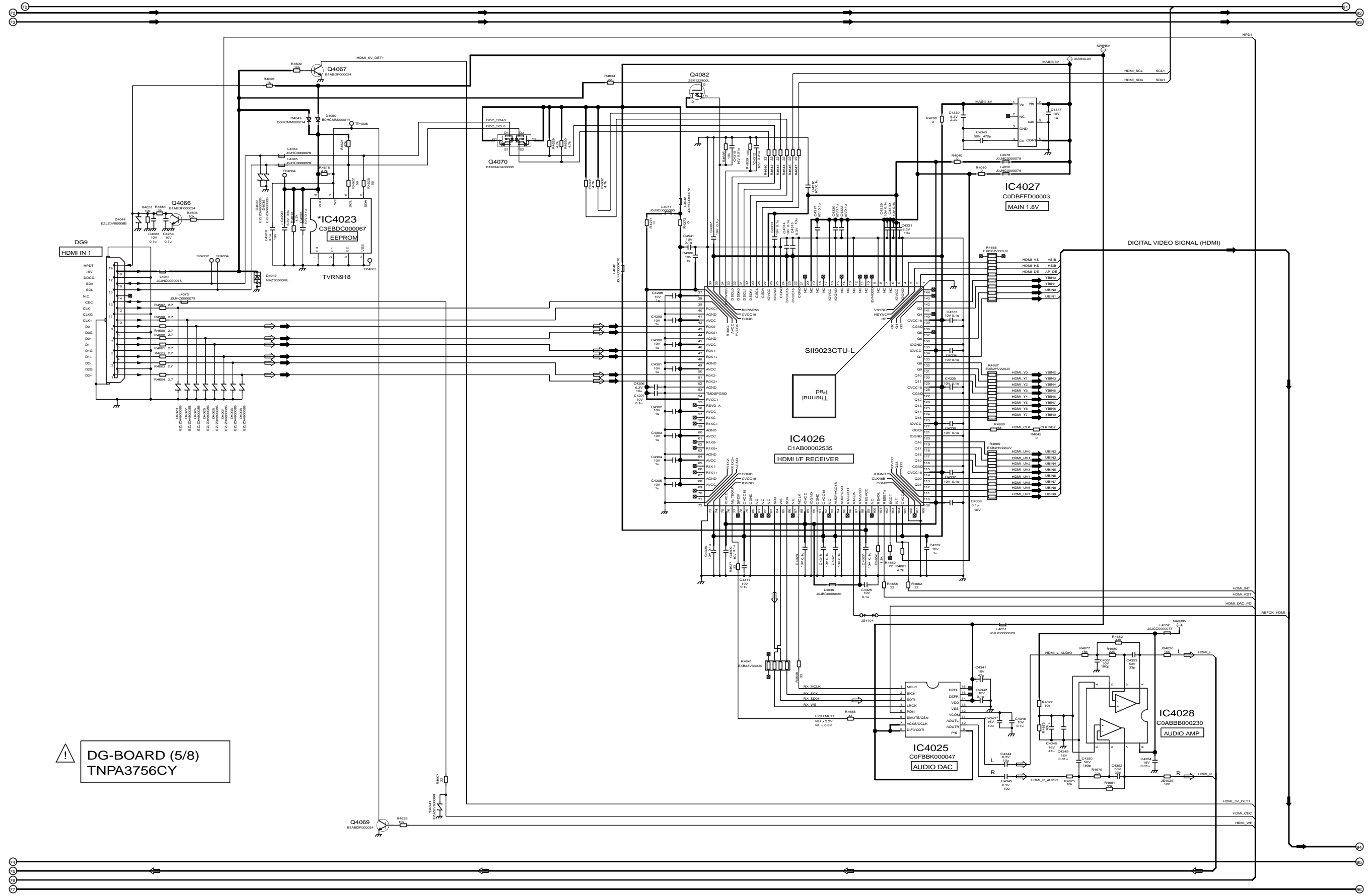
TH-42PA60L DG-Board (5 of 8) Schematic Diagram
