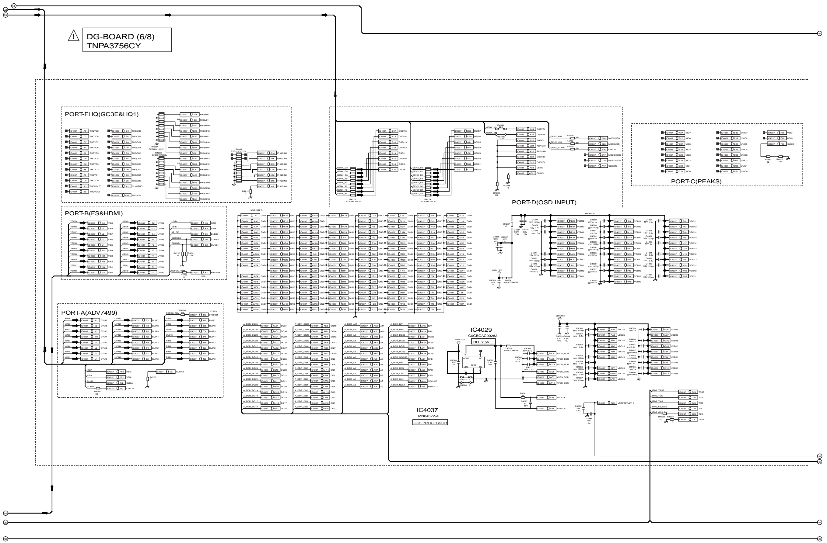
TH-42PA60L DG-Board (6 of 8) Schematic Diagram
