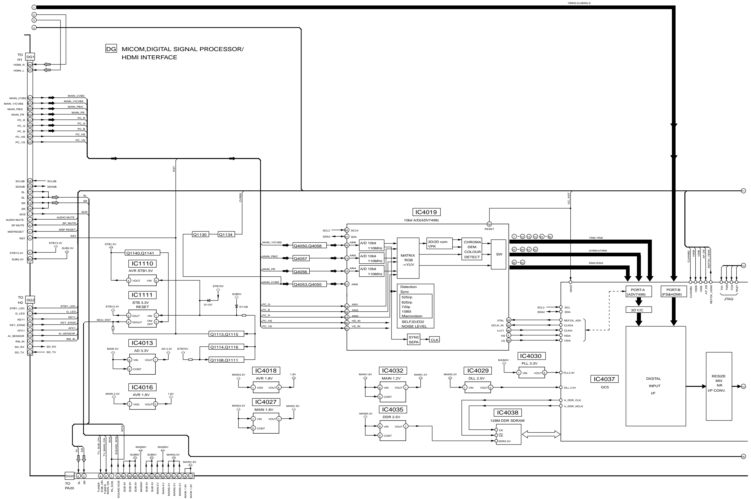
TH-42PA60L DG-Board (2 of 3) Block Diagram
