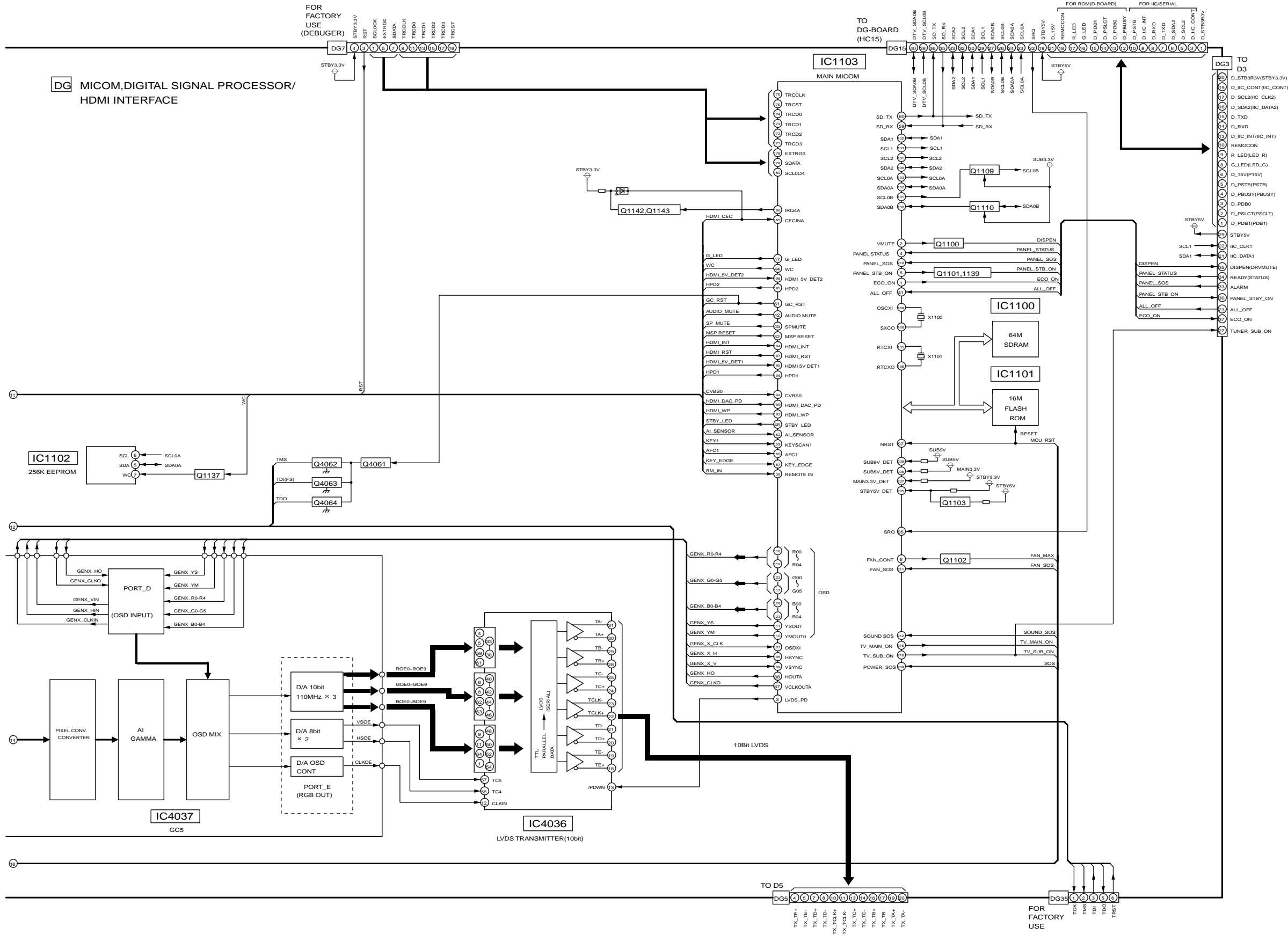
TH-42PA60L DG-BOARD (3 of 3) Block Diagram
