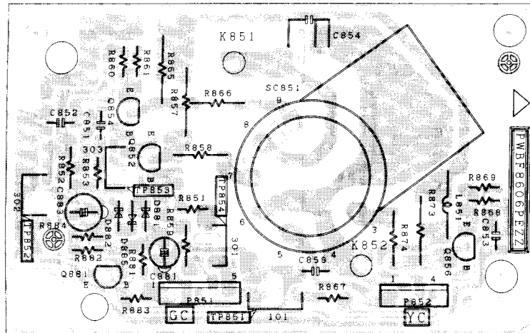
PWB-B
