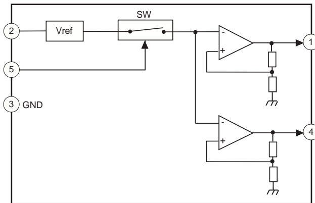
A BOARD IC604 BA41W12ST
