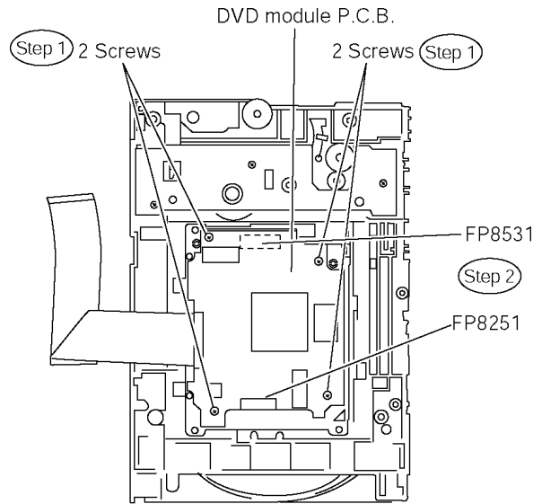
<Mechanism unit bottom>
