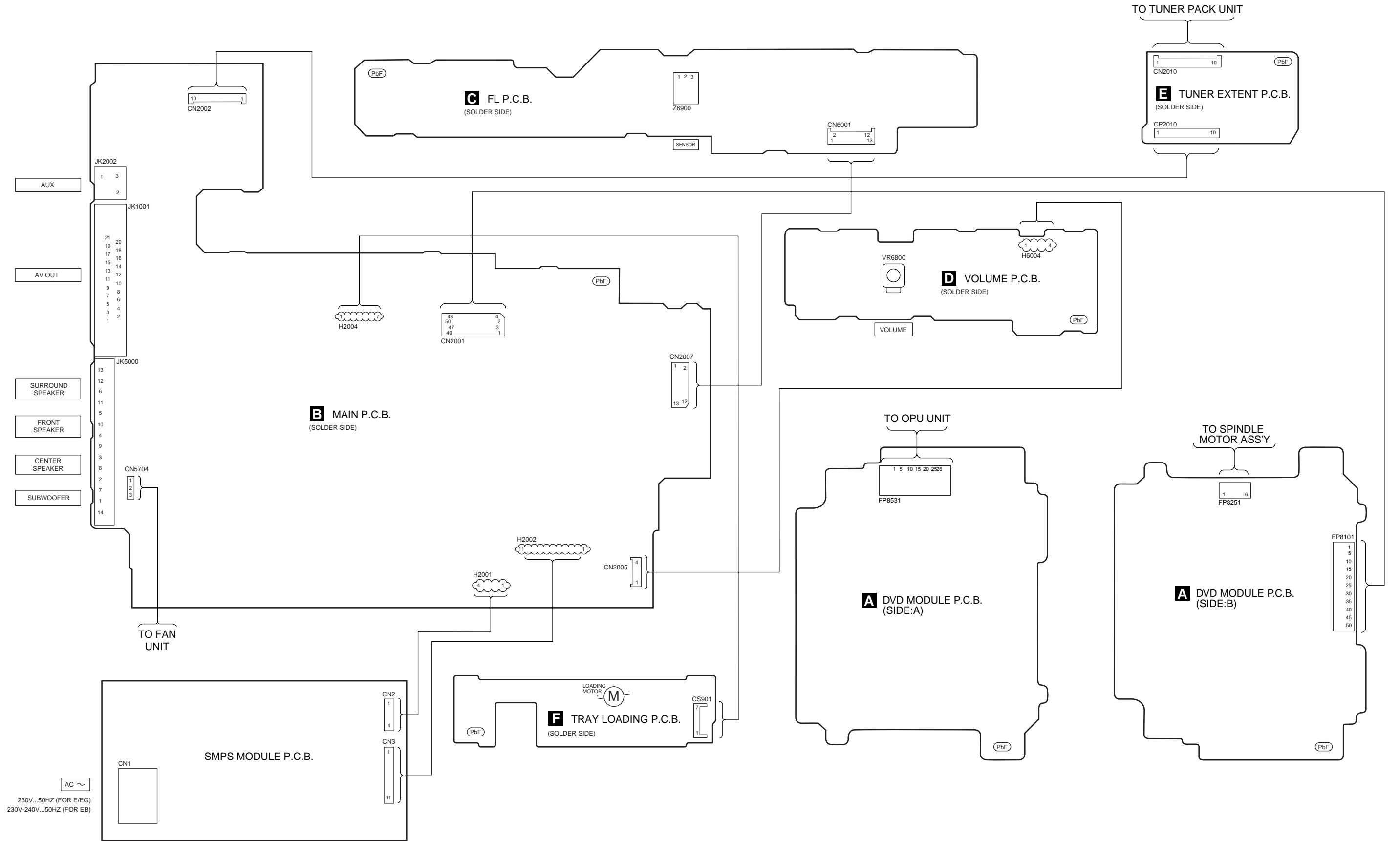
SA-HT340E/EB/EG WIRING CONNECTION
